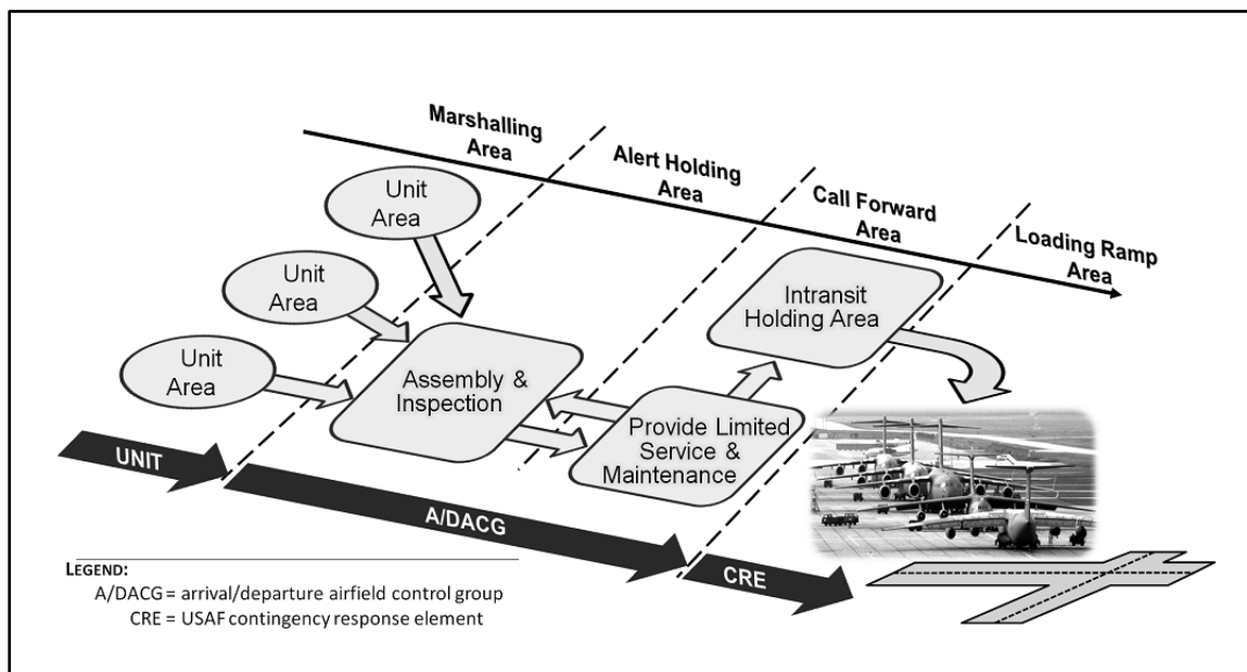
Figure 3-2. Notional Aerial Port of Embarkation (APOE)
